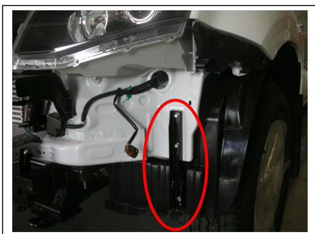
Figure 3: Passengers side outer bumper stiffener
